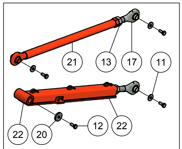
Detail B
